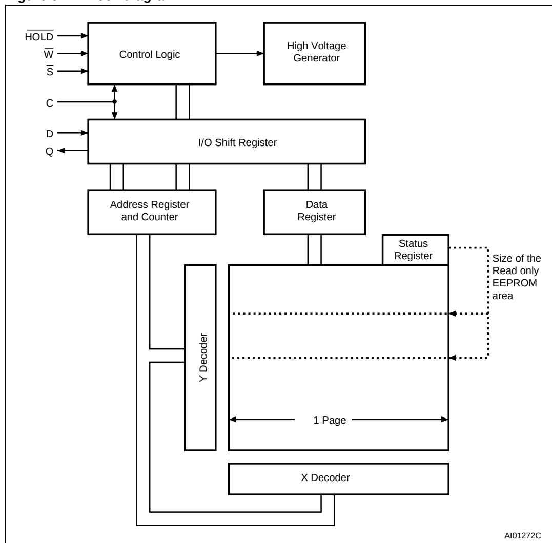
Figure 6. Block diagram
