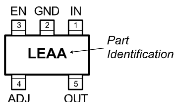
MIC5207BM5/YM5 (M5) (Adjustable Voltage)
