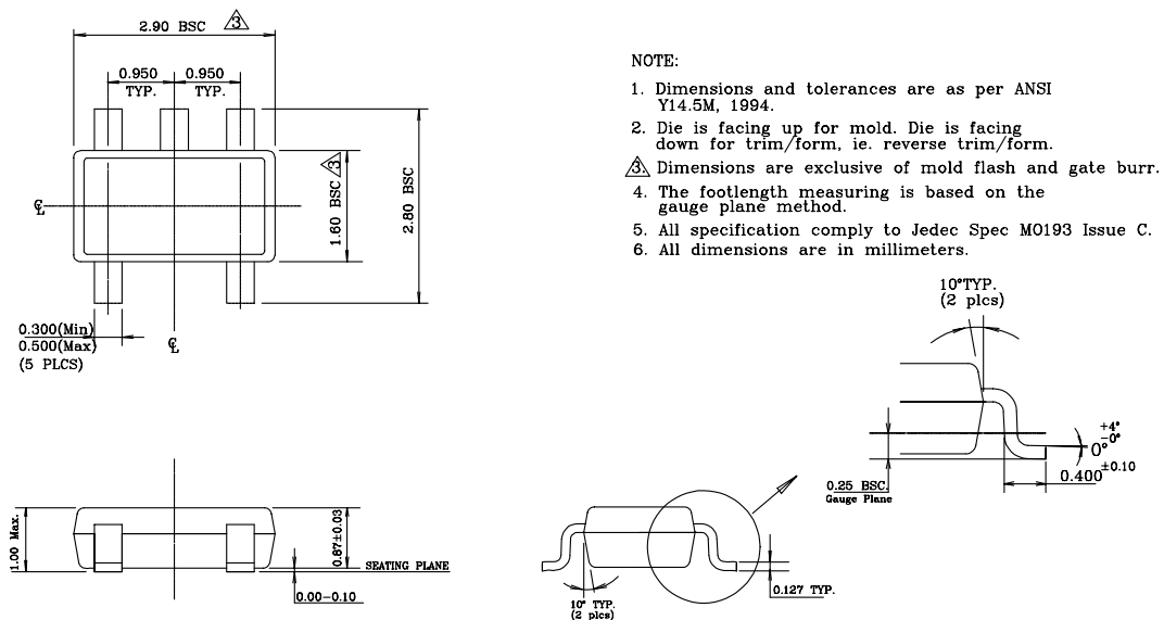
5-Pin Thin SOT-23 (D5)
