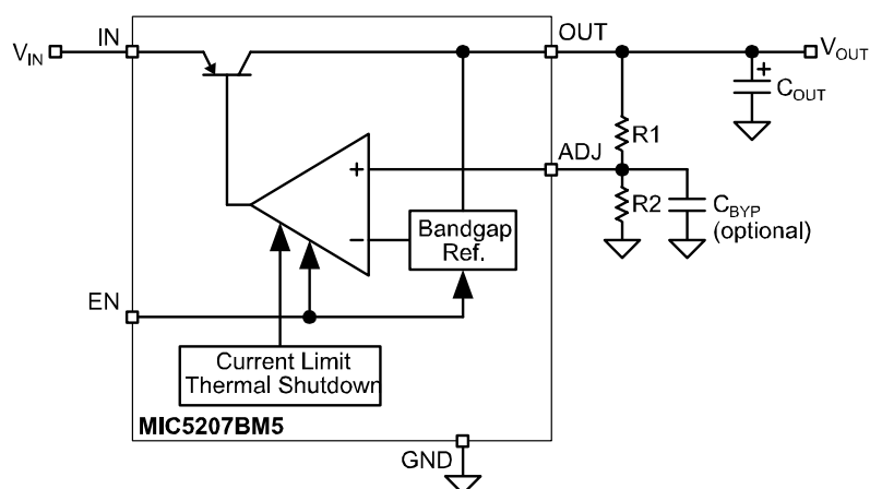
Ultra-Low-Noise Adjustable Regulator
