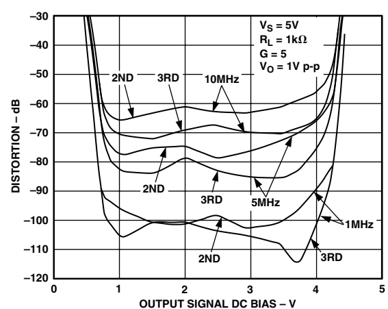
TPC 12. Harmonic Distortion vs. Output Signal DC Bias
