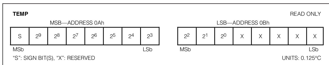
Figure 4. Temperature Register Format
