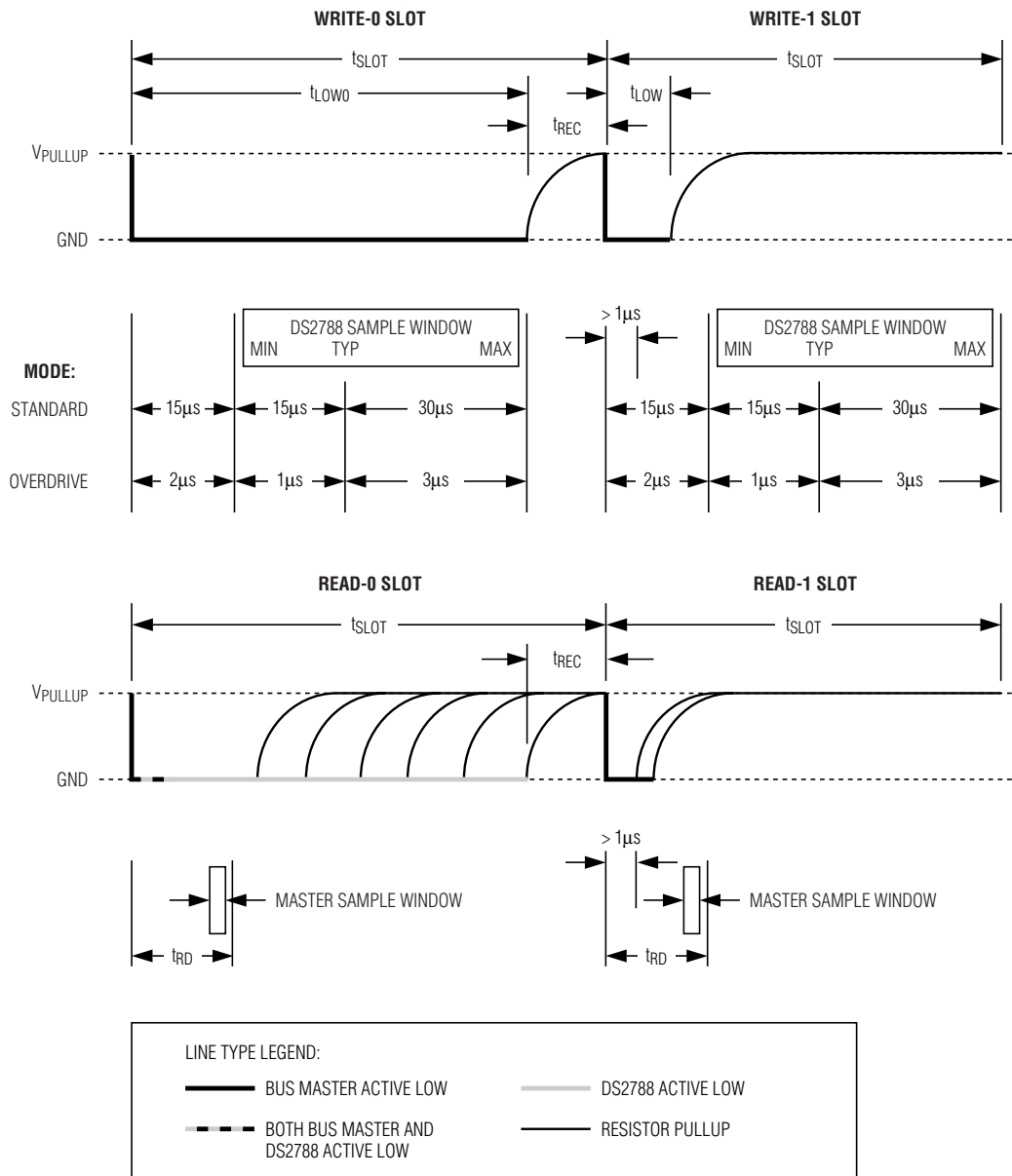
Figure 23. 1-Wire Write- and Read-Time Slots
