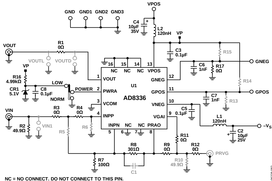
Figure 88. AD8336-EVALZ Schematic Shown as Shipped, Configured for a Noninverting Gain of 4×
