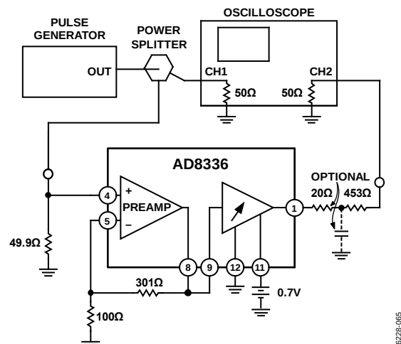
Figure 65. Pulse Response
