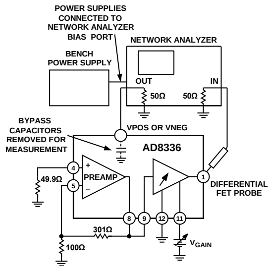
Figure 71. PSRR
