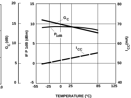
Figure 6. Typical Conversion Gain, IF P_{1dB} , and I_{CC} Current vs. Case Temperature, T_A = 25^\circ\text{C} , V_{CC} = 10\text{ V} , RF: -20 dBm at 2 GHz, LO: 0 dBm at 1.75 GHz.
