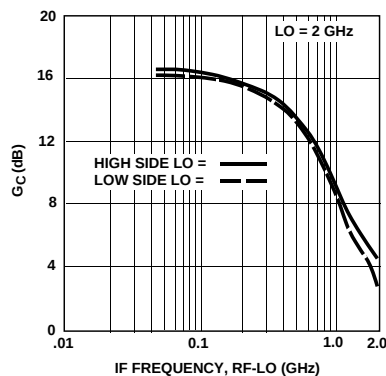
Figure 4. Typical RF to IF Conversion Gain vs. IF Frequency, T_A = 25^\circ\text{C} , V_{CC} = 10\text{ V} , LO: 0 dBm at 2 GHz.
