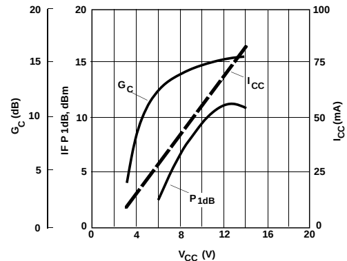
Figure 3. Typical Conversion Gain, IF P_{1dB} , and I_{CC} Current vs. V_{CC} Bias Voltage, T_A = 25^\circ\text{C} , RF: -20 dBm at 2 GHz, LO: 0 dBm at 1.75 GHz.
