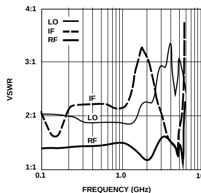
Figure 5. RF, LO, and IF Port VSWR vs. Frequency, T_A = 25^\circ\text{C} , V_{CC} = 10\text{ V} .
