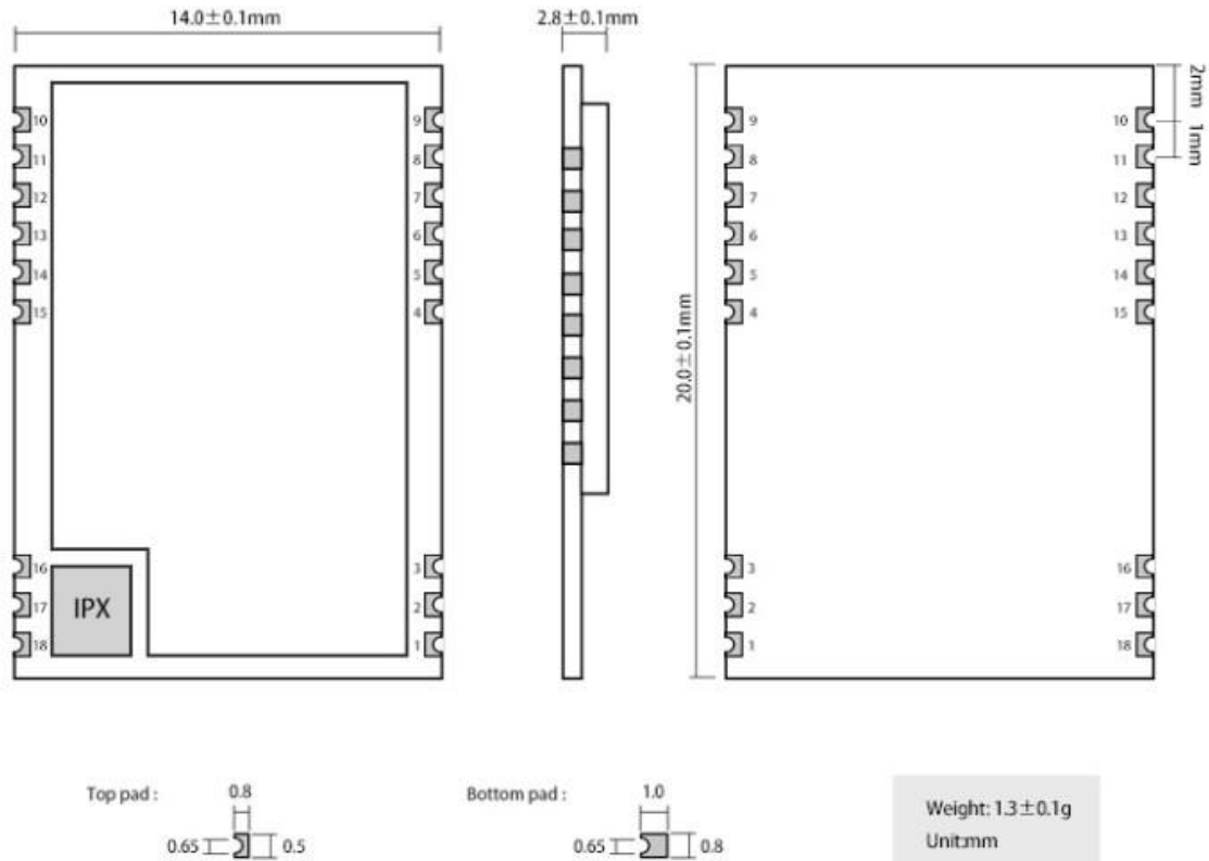
Figure 3-1 Dimensions and pin definitions
