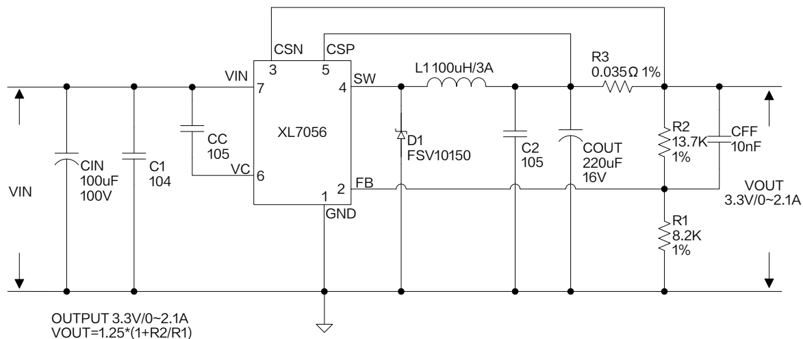
Figure11. XL7056 System Application (VOUT=3.3V, IOU=0~2.1A)
