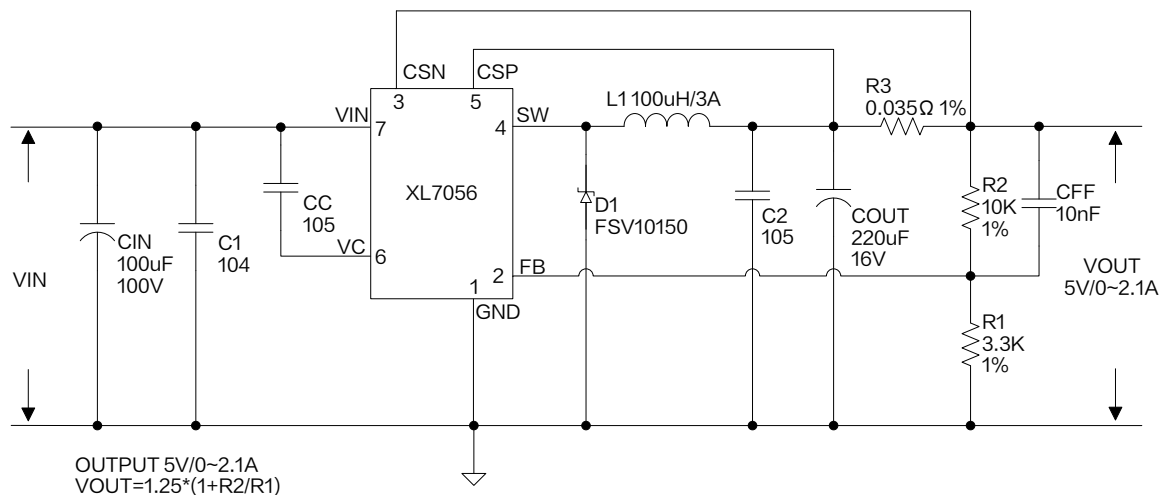
Figure9. XL7056 System Application (VOUT=5V, IOUT=0~2.1A)
