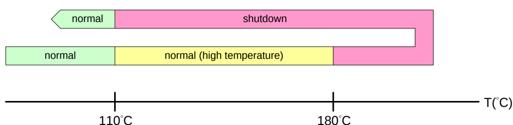
Relations between Thermal Shutdown and Junction Temperature
