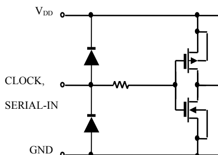
3. CLOCK, SERIAL-IN terminal
