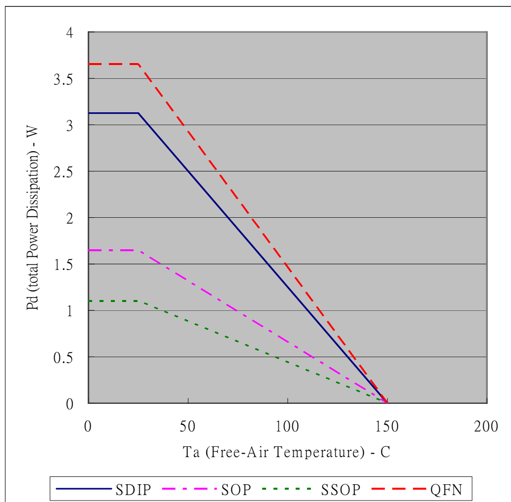
Figure 9. Power Dissipation vs. Operating Temperature
