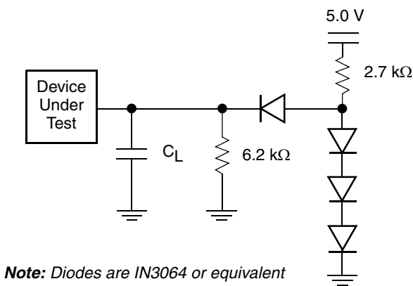
Figure 7. Test Setup
