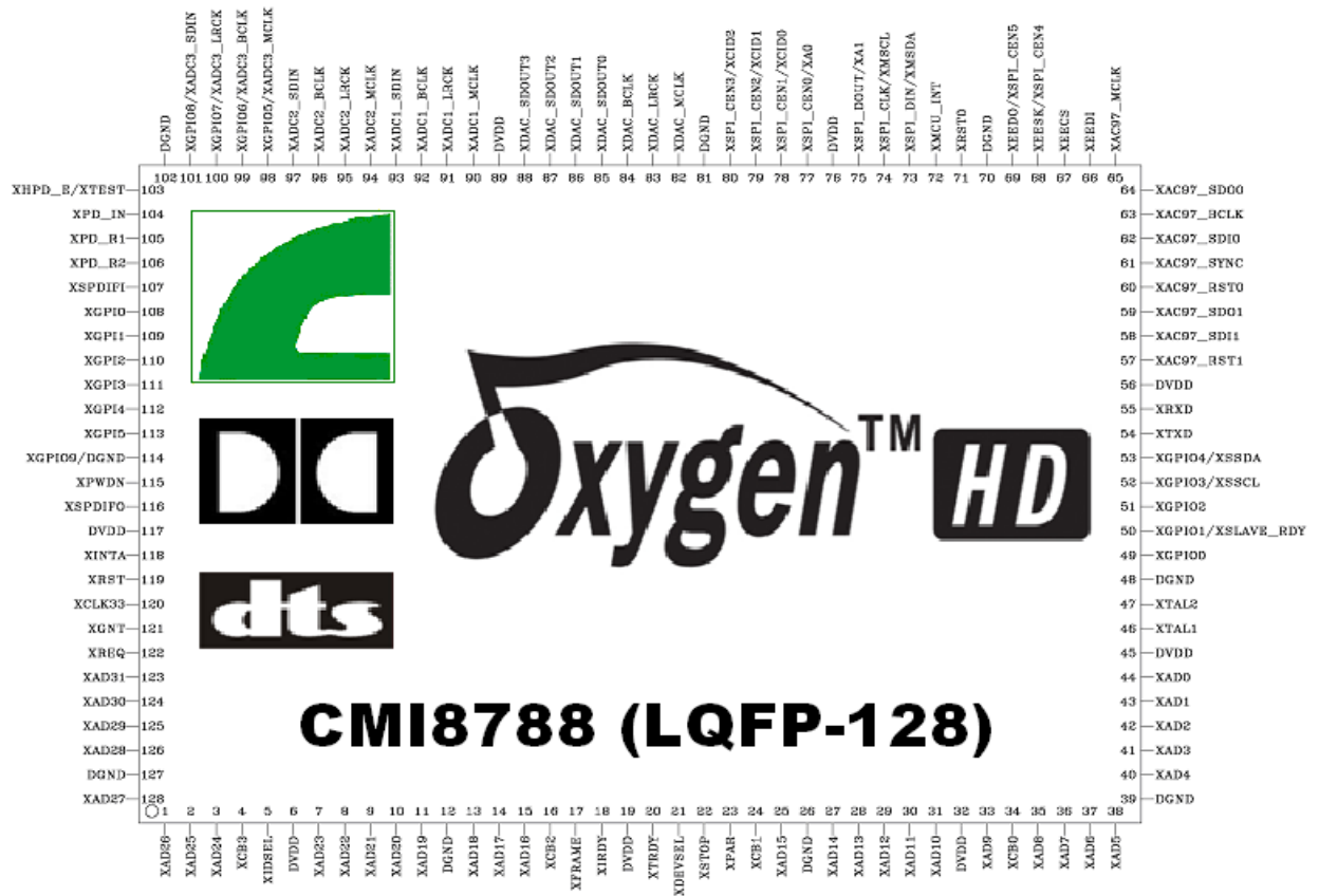
Figure 2. Pinout Diagram of Oxygen™HD CMI8788
