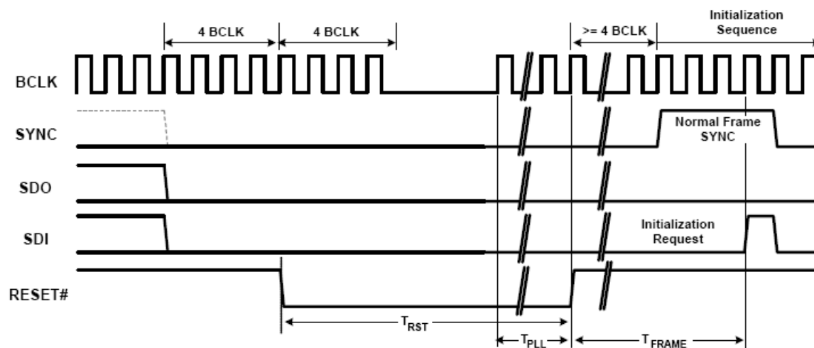
Link Reset and Initialization Timing
