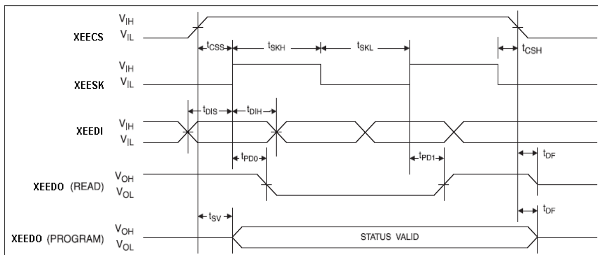
EEPROM Interface Timing Diagram
