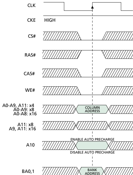
Figure 13 WRITE Command
