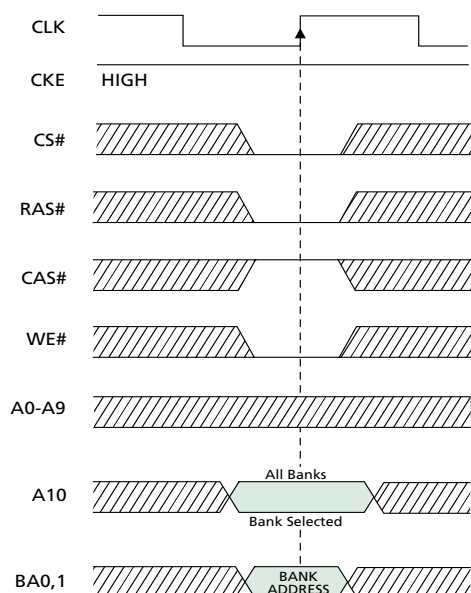
Figure 20 PRECHARGE Command
