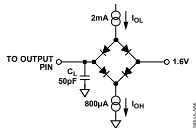
Figure 5. Load Circuit for Timing Specifications
