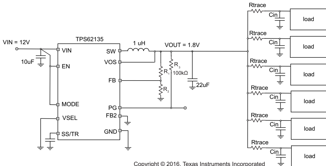
Figure 75. Multiple Loads
