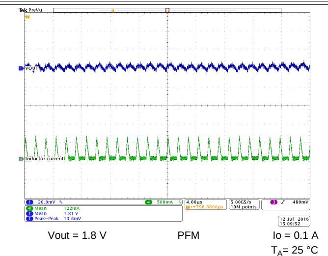
Figure 43. Output Voltage Ripple
