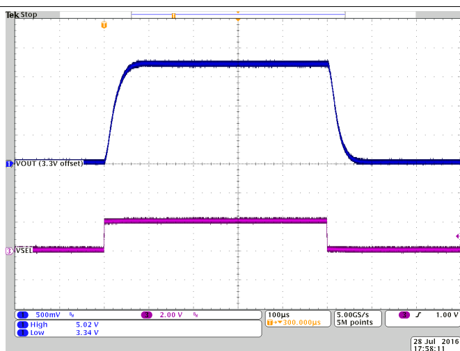
Figure 73. Output Voltage Change from 3.3 V to 5 V in PWM with 20 Ω load resistance
