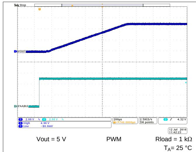
Figure 56. Start-Up Timing
