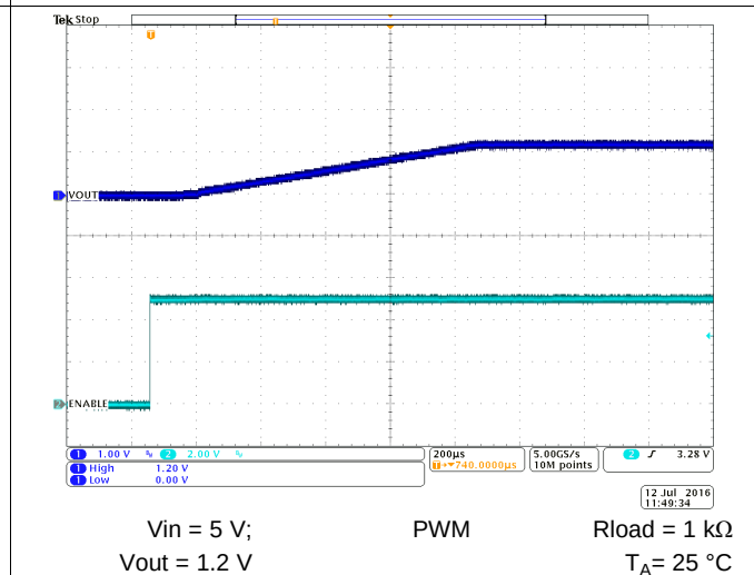
Figure 35. Start-Up Timing
