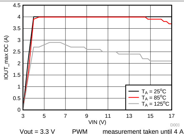
Figure 28. Maximum Output Current vs Input Voltage
