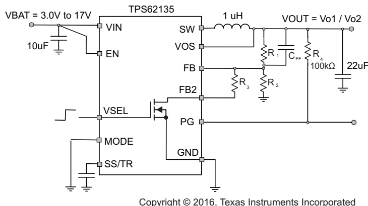
Figure 71. Typical Application using VSEL
