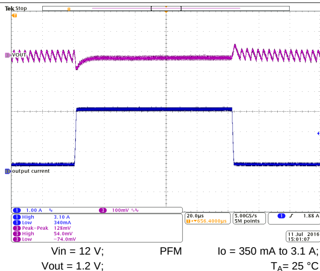
Figure 31. Load Transient Response
