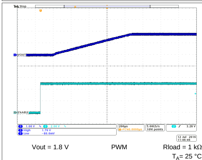
Figure 42. Start-Up Timing
