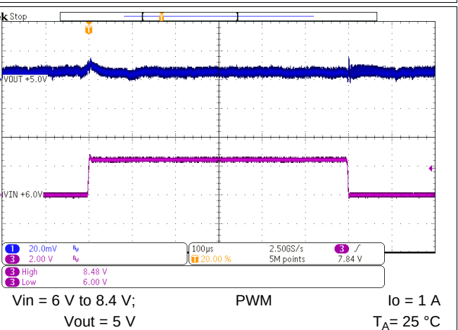
Figure 55. Line Transient Response
