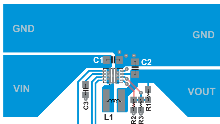
Figure 80. Layout
