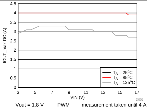
Figure 27. Maximum Output Current vs Input Voltage
