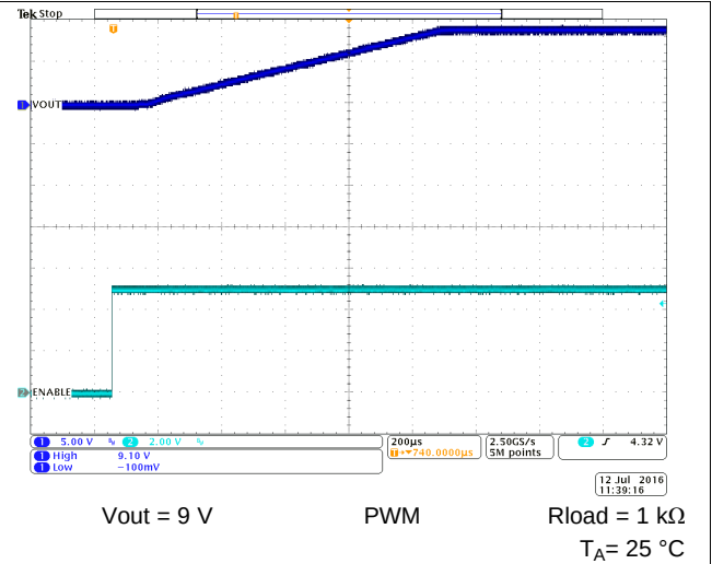
Figure 63. Start-Up Timing
