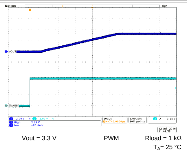
Figure 49. Start-Up Timing
