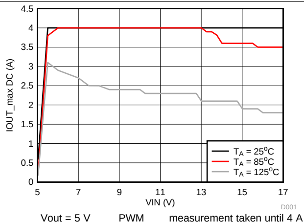
Figure 29. Maximum Output Current vs Input Voltage
