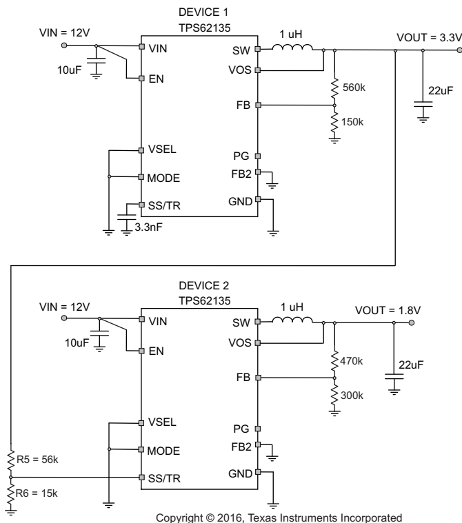
Figure 76. Tracking Example
