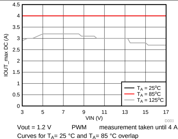
Figure 26. Maximum Output Current vs Input Voltage
