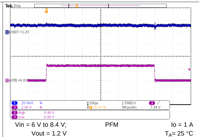
Figure 33. Line Transient Response
