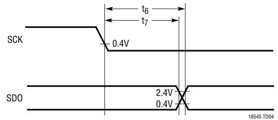
t_6 (Delay Time, SCK \square to SDO Valid) t_7 (Time from Previous Data Remains Valid After SCK \square )
