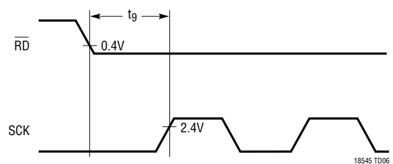
t_9 ( \overline{RD} \square to SCK Setup Time)
