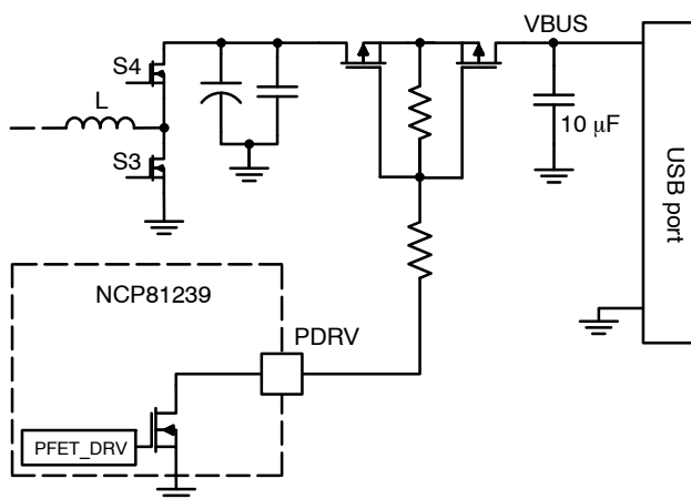
Figure 12. PFET Drive
